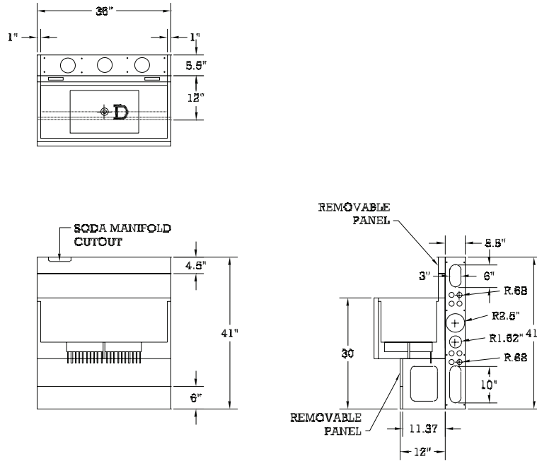
Bar Sink Side View
