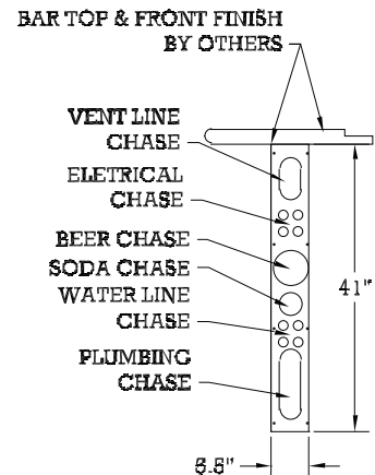
Flat Wall Side View
