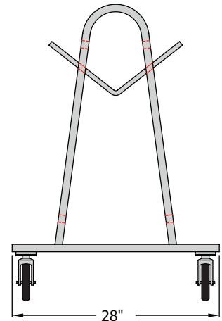
99360 All-Welded Cart
