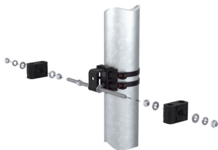
Threaded Rod Adapter with Universal Round Member base 900638-10
