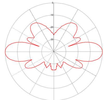
Vertical, 0° Downtilt
