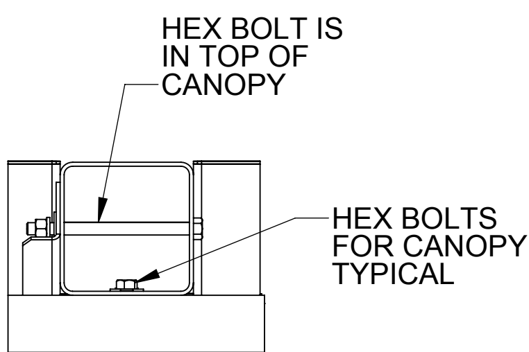
SECTION F-F SCALE 1 : 4
