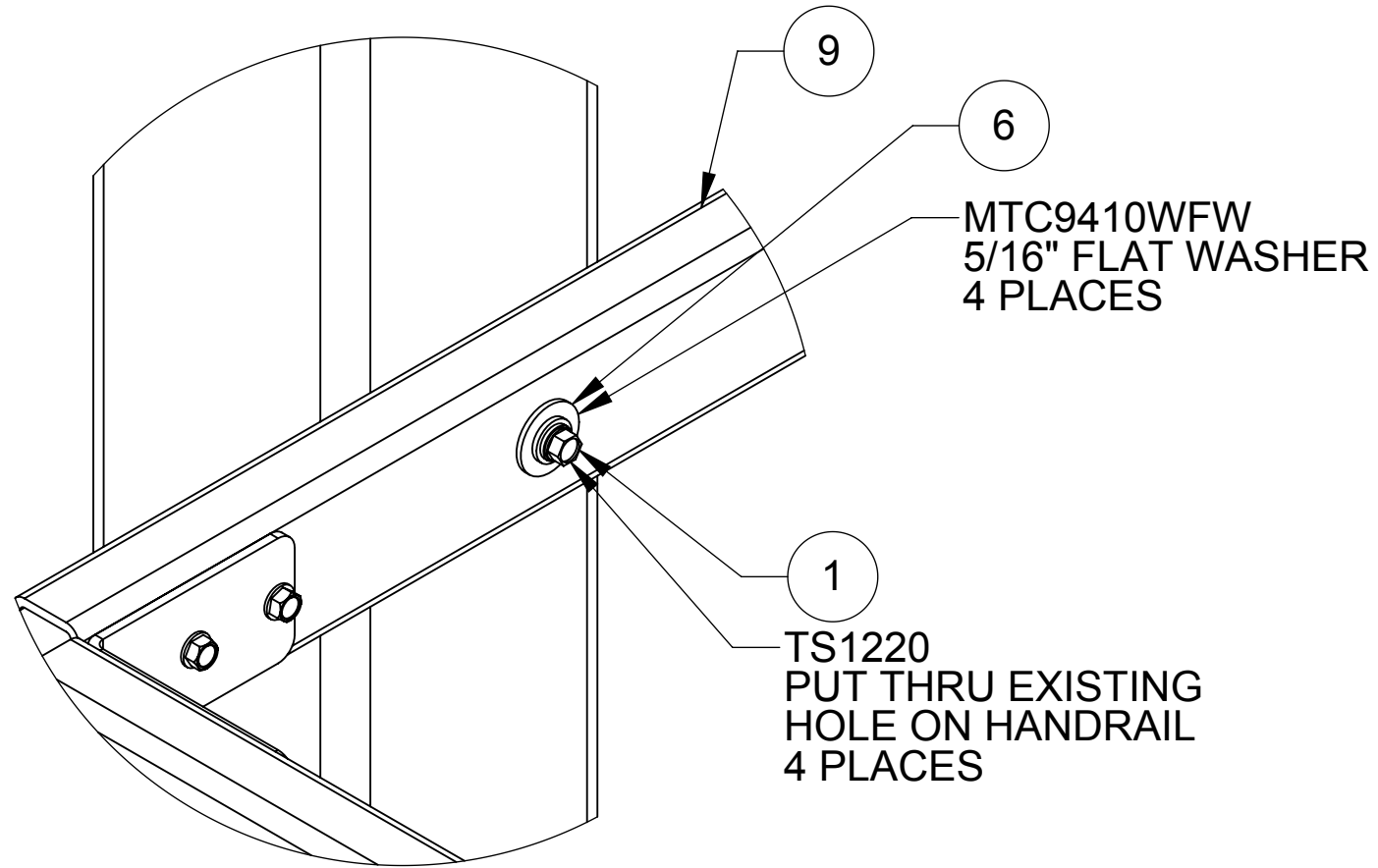
DETAIL J SCALE 1:2
