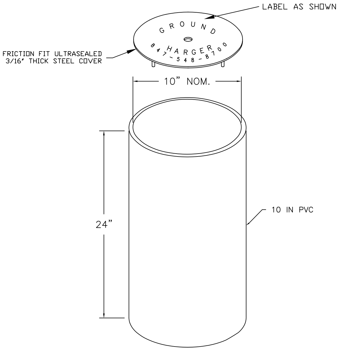
PVC WELL W/ STEEL COVER
