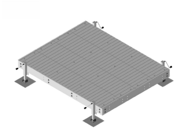
E20® Equipment Platform, 8 ft x 10 ft, base with four adjustable legs
